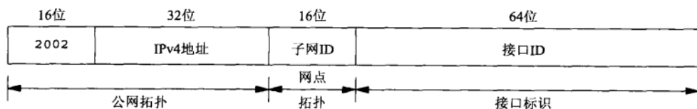
图B-3 6to4地址
