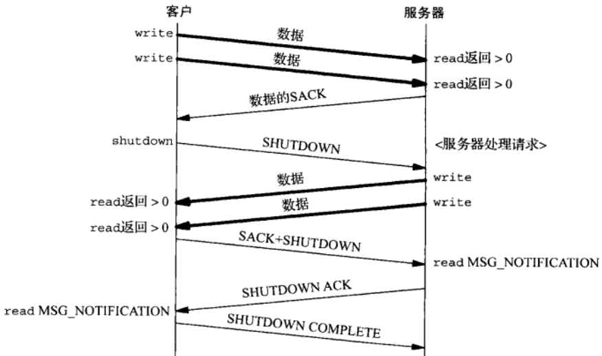
图9-5 调用shutdown关闭一个SCTP关联
