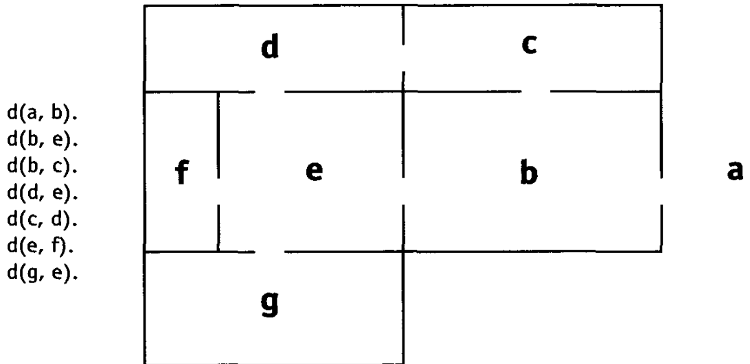
Fig. 7.1. A floor plan and the program that represents it
