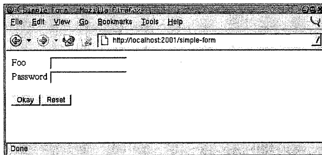
图26-5 http://localhost:2001/simple-form
