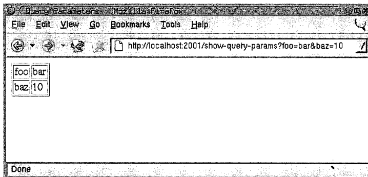
图26-4 http://localhost:2001/show-query-params?foo=bar&baz=10
