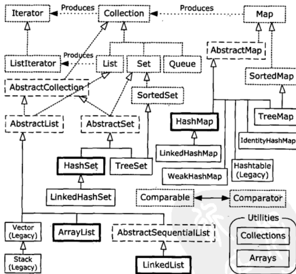
Full Container Taxonomy
