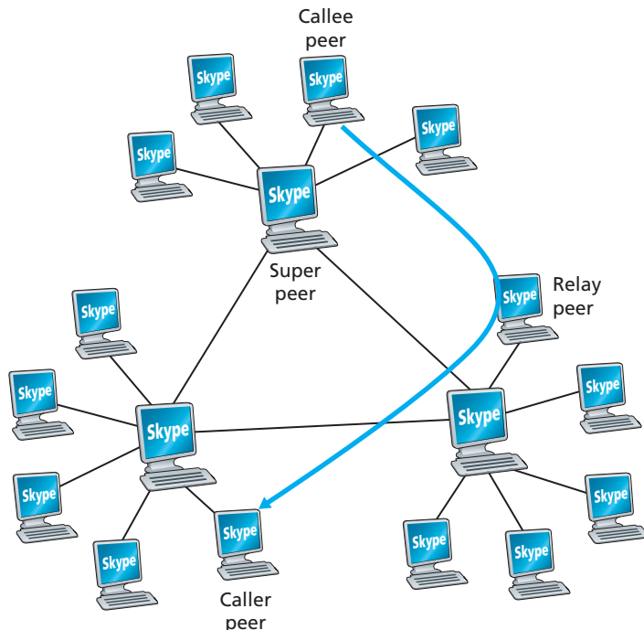
Figure 7.10 ♦ Skype peers
