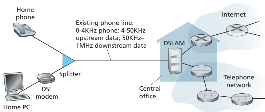
Figure 1.6 ♦ DSL Internet access
