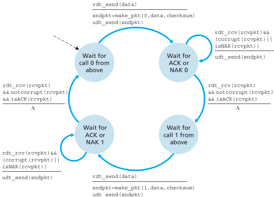
Figure 3.11 ♦ rdt2.1 sender
