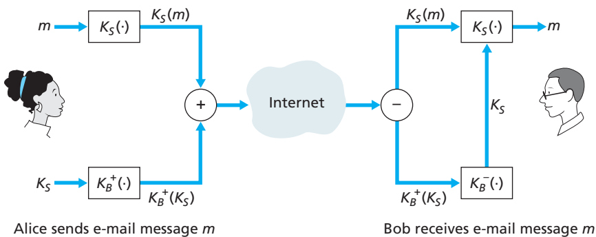
Figure 8.20 ♦ Alice used a symmetric session key, K_S , to send a secret e-mail to Bob.
