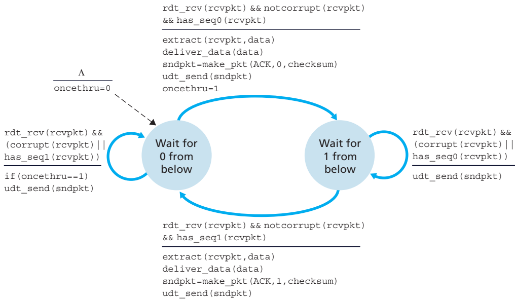
Figure 3.14 ♦ rdt2.2 receiver
