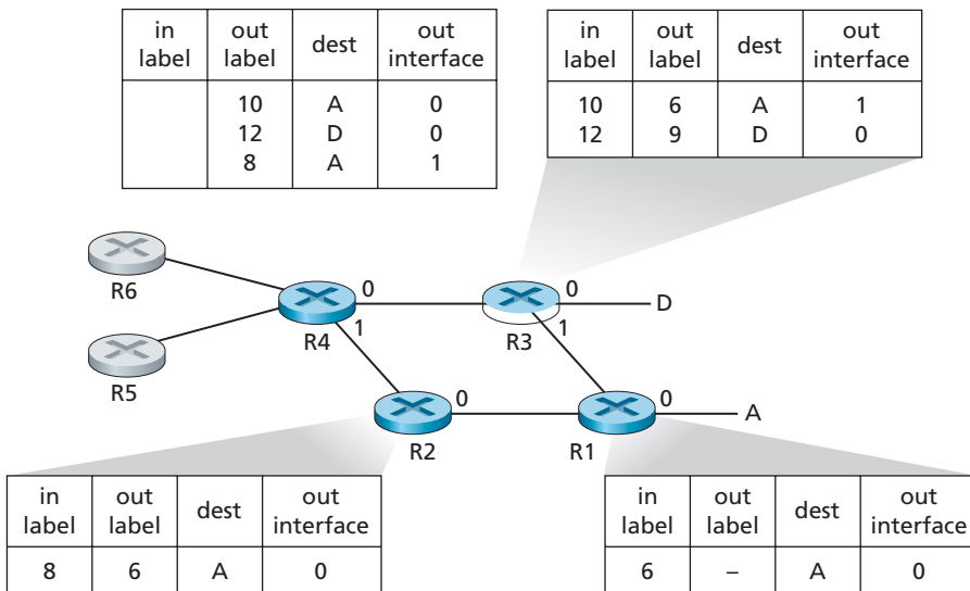
Figure 5.36 ♦ MPLS-enhanced forwarding
