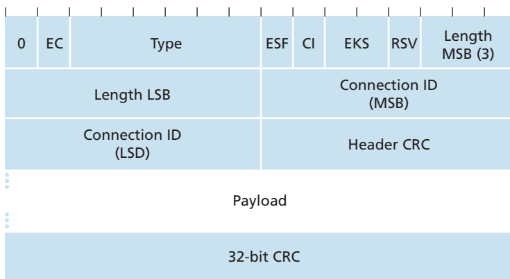
Figure 6.18 ♦ 802.16 packet
