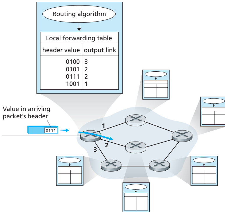
Figure 4.2 ♦ Routing algorithms determine values in forwarding tables.
