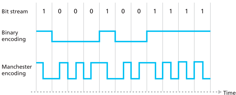
Figure 5.23 ♦ Manchester encoding
