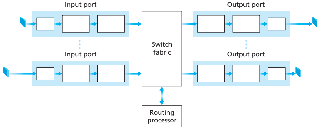
Figure 4.6 ♦ Router architecture
