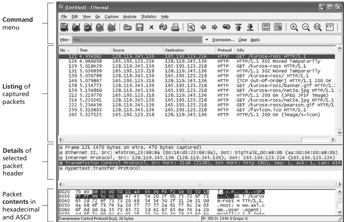
Figure 1.29 ♦ A Wireshark screen shot
