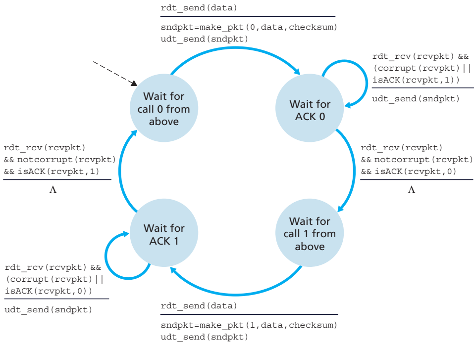
Figure 3.13 ♦ rdt2.2 sender
