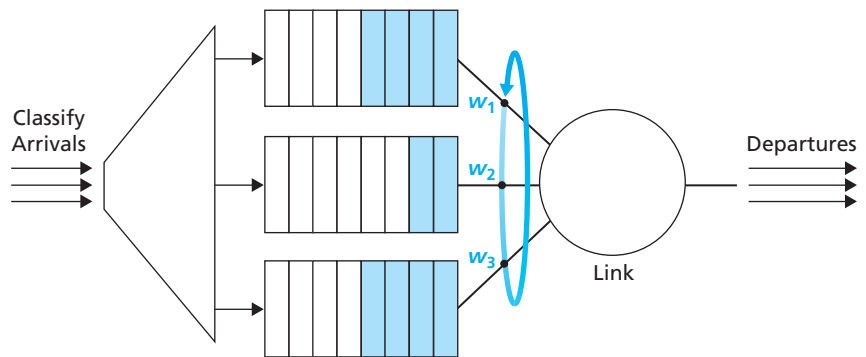
Figure 7.26 ♦ Weighted fair queuing (WFQ)
