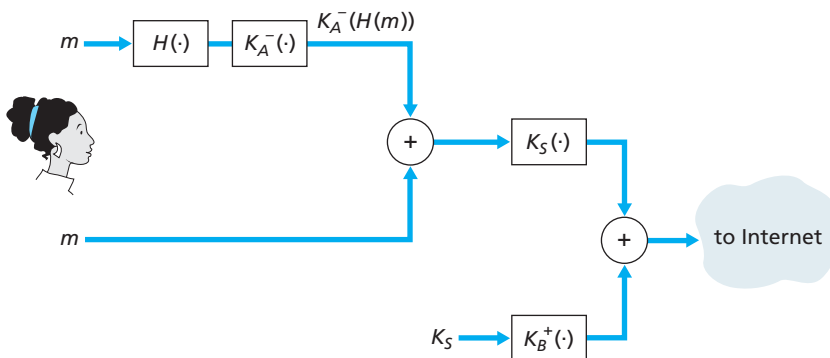
Figure 8.22 ♦ Alice uses symmetric key cryptography, public key cryptography, a hash function, a digital signature to provide secrecy, sender authentication, and message integrity.
