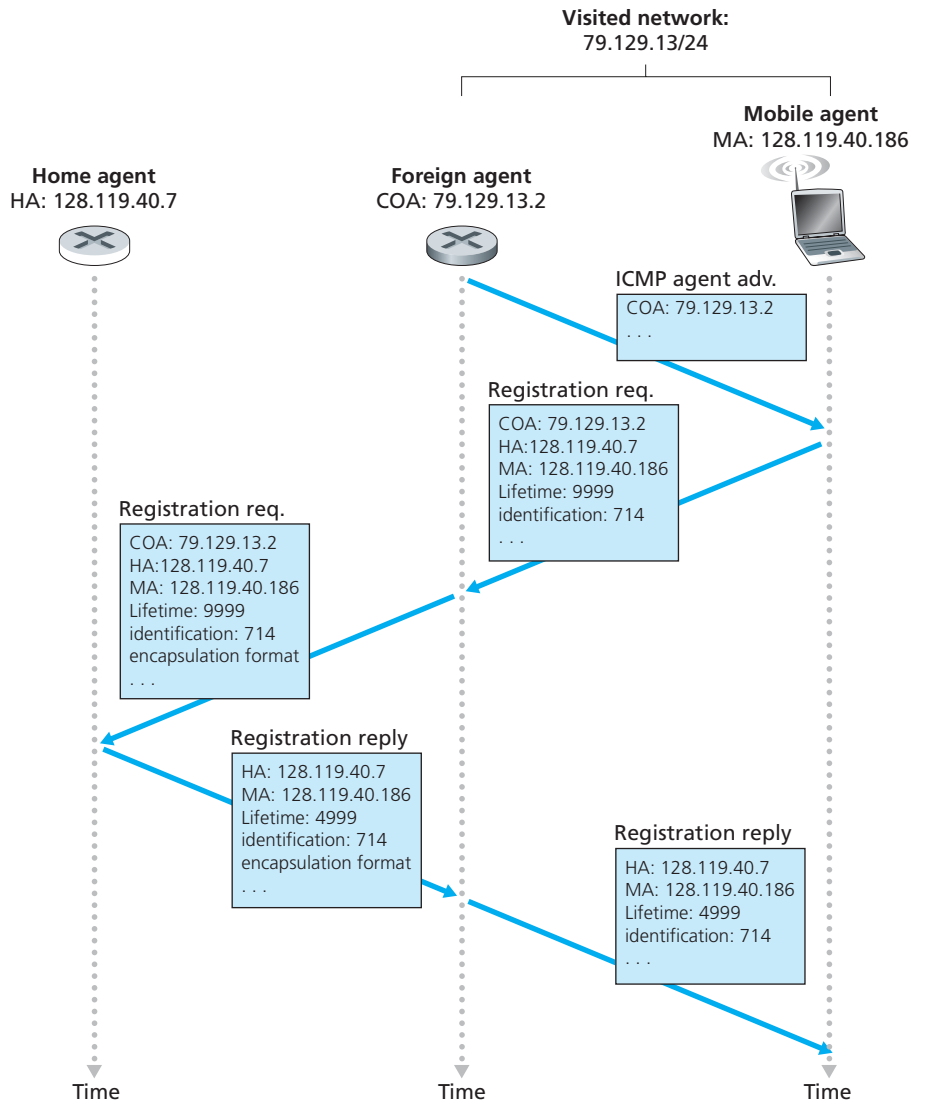
Figure 6.28 ♦ Agent advertisement and mobile IP registration
