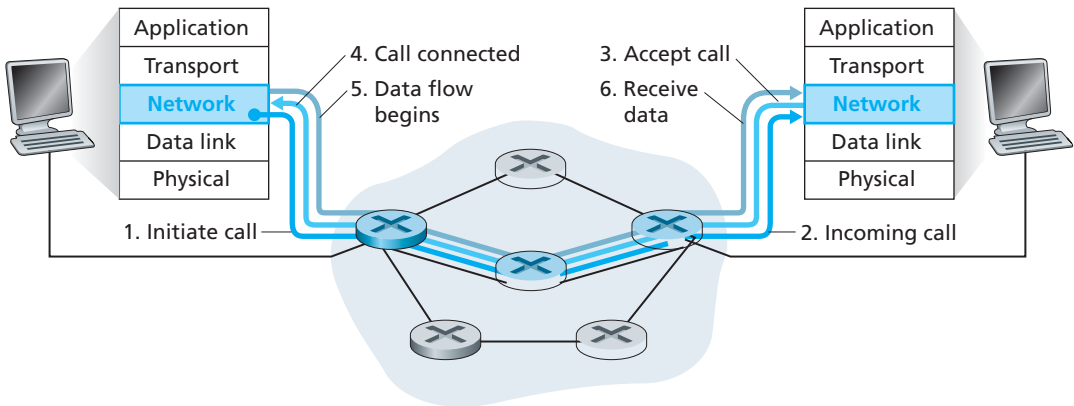
Figure 4.4 ♦ Virtual-circuit setup
