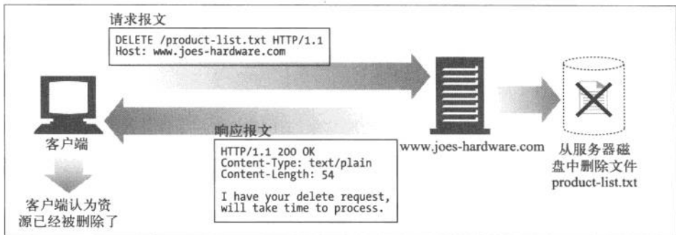
图 3-13 DELETE 示例
