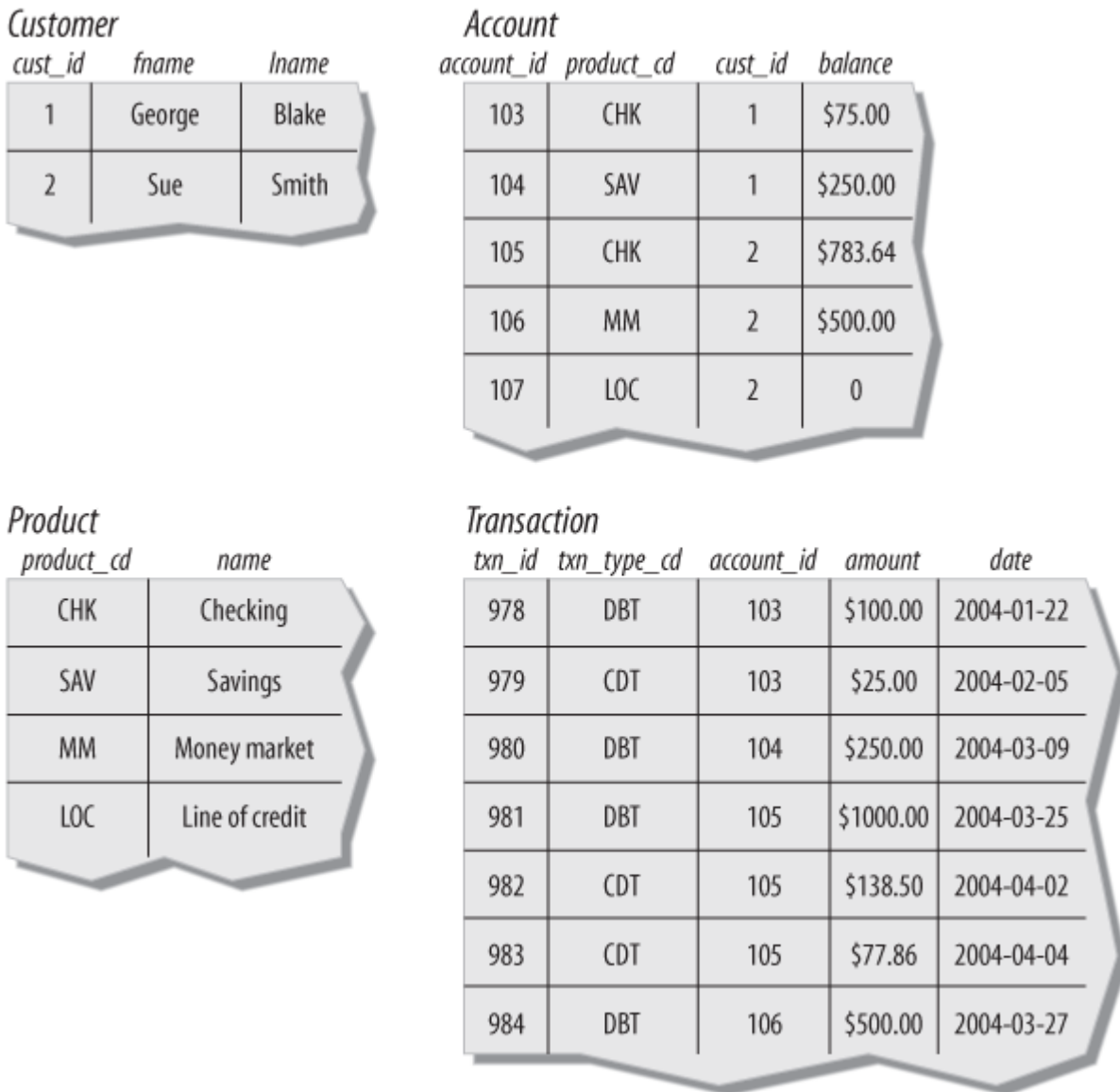
Figure 1-3. Relational view of account data
