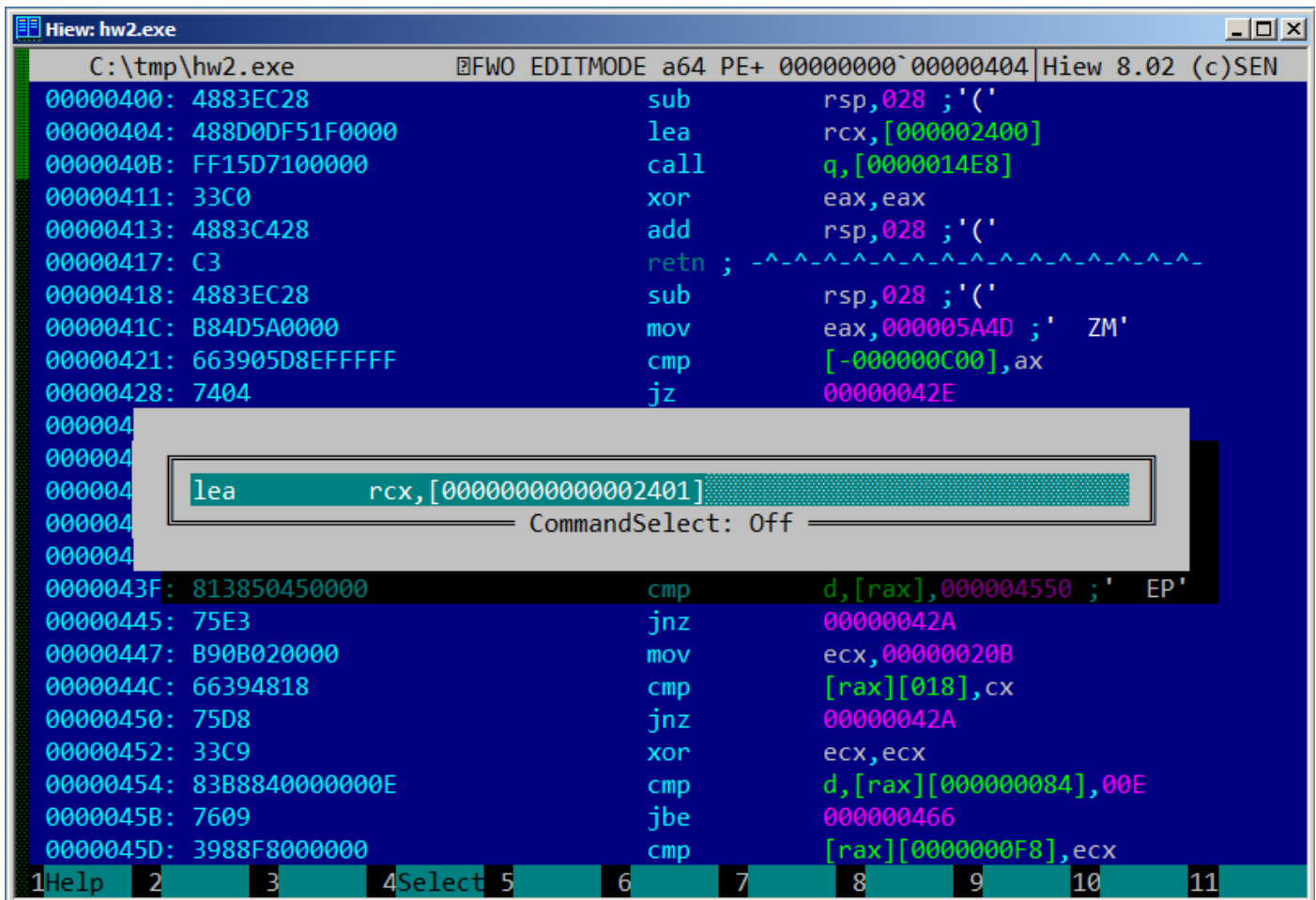
Figure 1.3: Hiew
