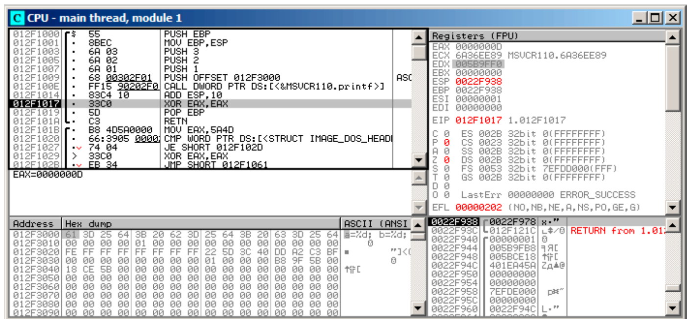
Figure 1.11: OllyDbg: after ADD ESP, 10 instruction execution
