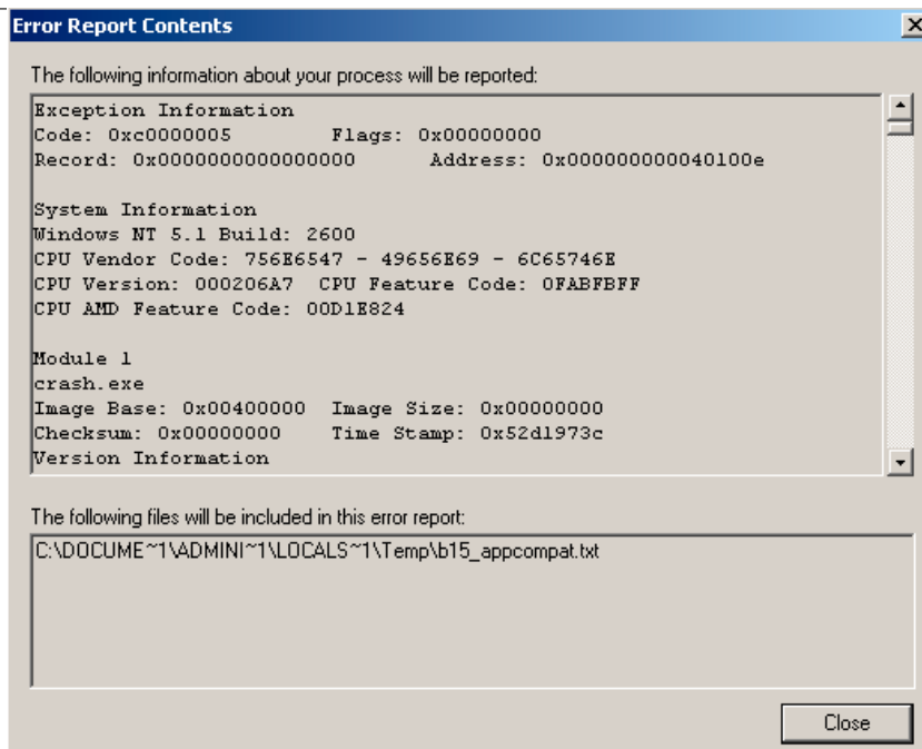
Figure 6.3: Windows XP
