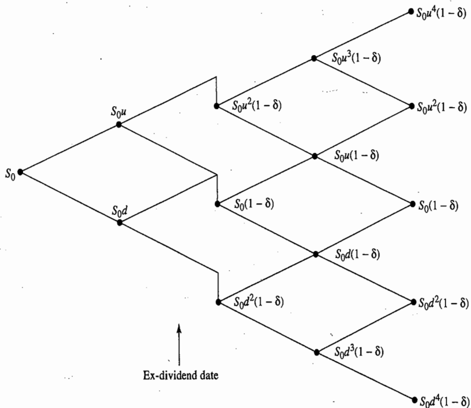
Figure 19.7 Tree when stock pays a known dividend yield at one particular time.
