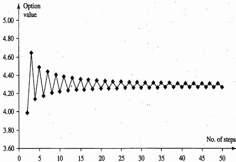
Figure 19.4 Convergence of the price of the option in Example 19.1 calculated from the DerivaGem Application Builder functions.
