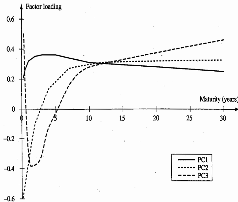
Figure 20.6 The three most important factors driving yield curve movements.
