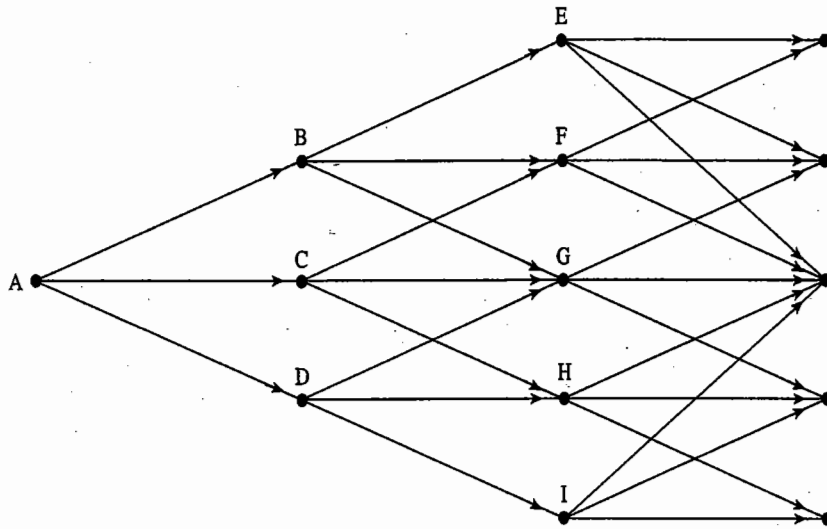
Figure 30.8 Tree for R^* in Hull-White model (first stage).
