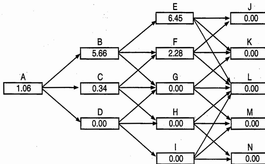
Figure 33.5 Valuation of option to expand the project: p_u , p_m , and p_d are the probabilities of “up”, “middle”, and “down” movements from a node.
