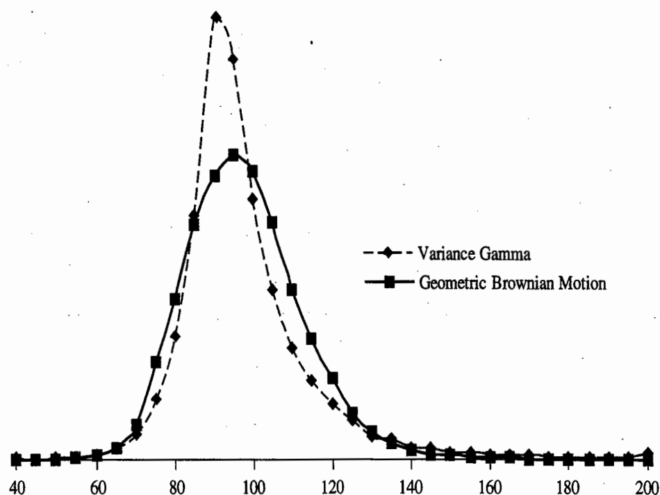
Figure 26.1 Distributions obtained with variance-gamma process and geometric Brownian motion.
