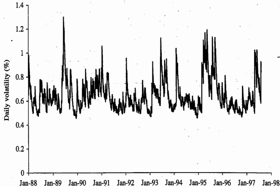
Figure 21.1 Daily volatility of the yen/USD exchange rate, 1988–1997.
