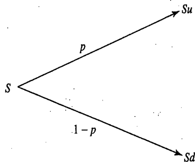
Figure 19.1 Asset price movements in time \Delta t under the binomial model.
