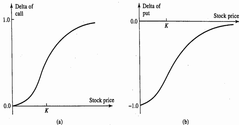
Figure 17.3 Variation of delta with stock price for (a) a call option and (b) a put option on a non-dividend-paying stock.
