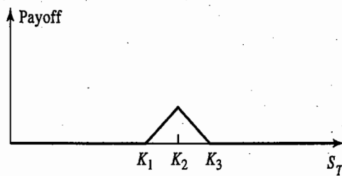
Figure 10.13 “Spike payoff” from a butterfly spread that can be used as a building block to create other payoffs.
