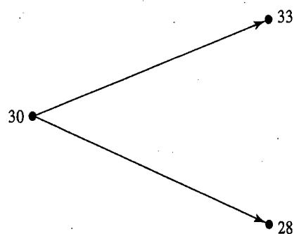
Figure 16.1 Futures price movements in numerical example.
