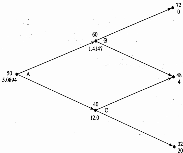
Figure 11.8 Using a two-step tree to value an American put option. At each node, the upper number is the stock price and the lower number is the option price.
