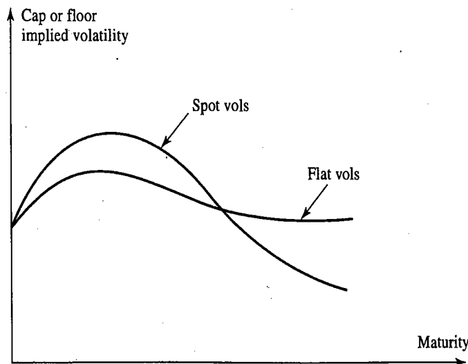
Figure 28.3 The volatility hump.
