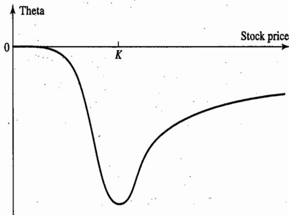
Figure 17.5 Variation of theta of a European call option with stock price.
