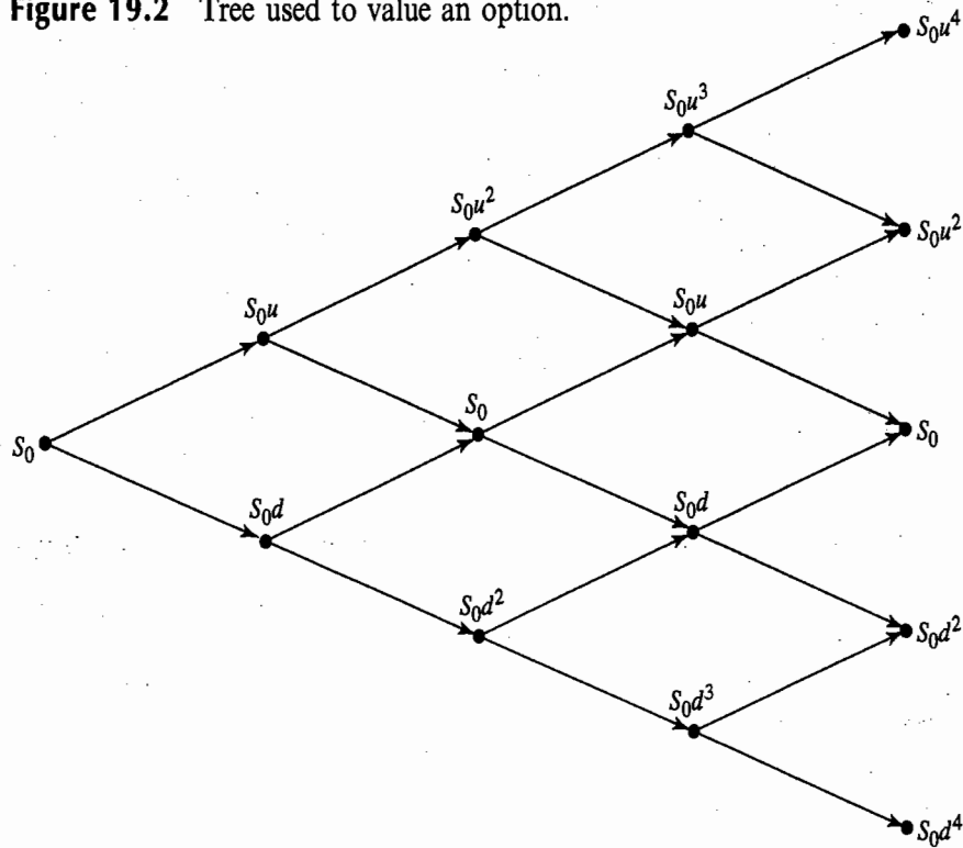
Figure 19.2 Tree used to value an option.
