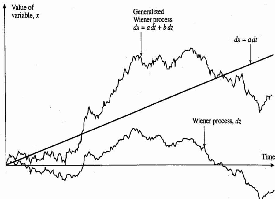
Figure 12.2 Generalized Wiener process with a = 0.3 and b = 1.5 .
