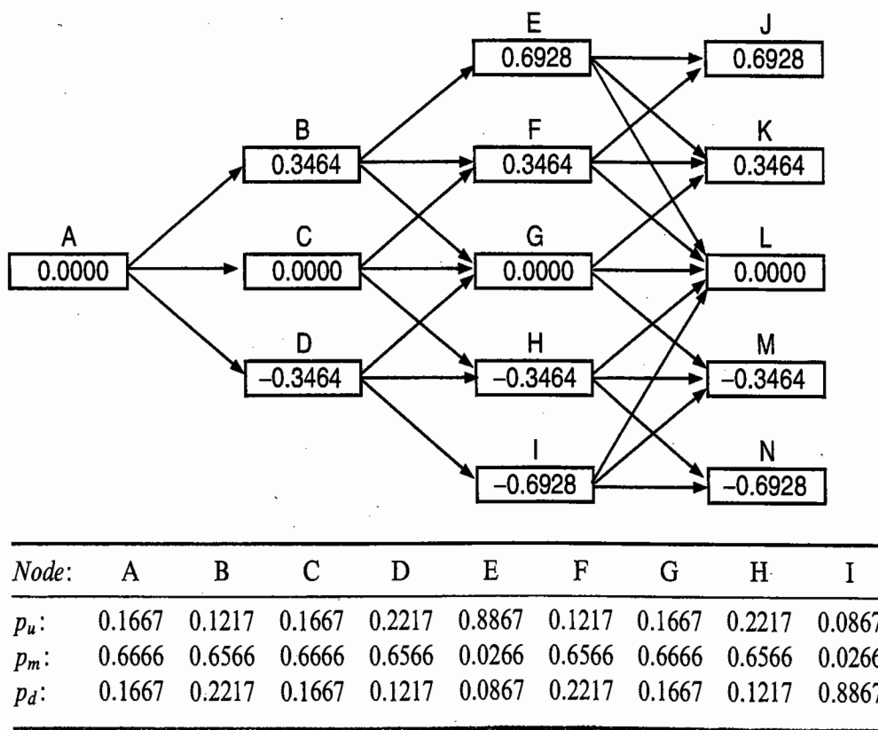
Figure 33.1 Tree for X . Constructing this tree is the first stage in constructing a tree for the spot price of a commodity, S . Here p_u , p_m , and p_d are the probabilities of “up”, “middle”, and “down” movements from a node.
