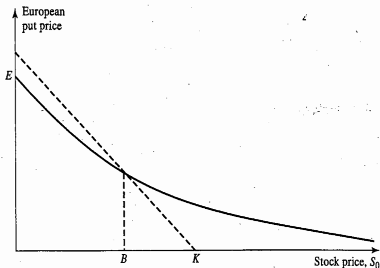
Figure 9.5 Variation of price of a European put option with the stock price, S_0 .
