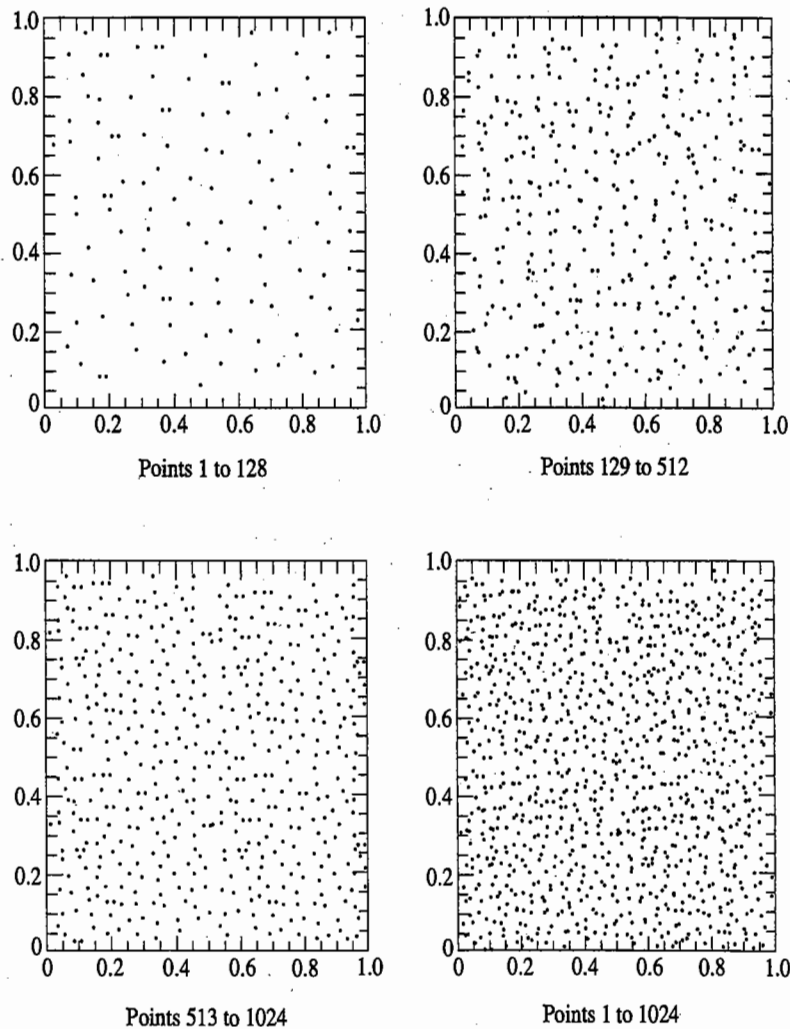
Figure 19.14 First 1024 points of a Sobol' sequence.
