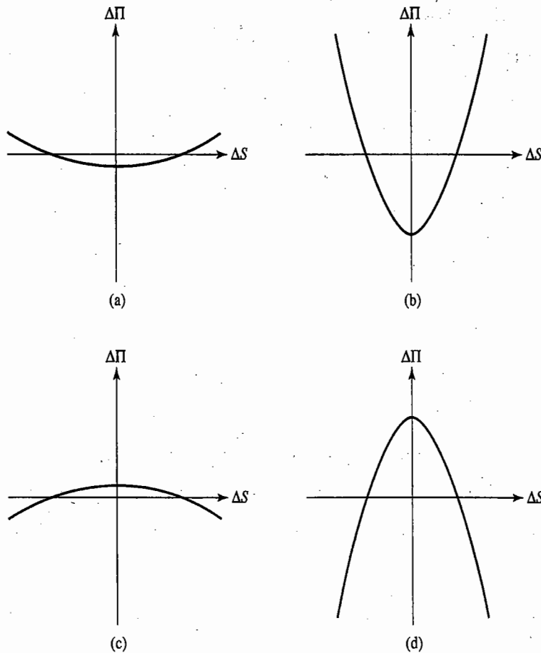
Figure 17.8 Relationship between \Delta\Pi and \Delta S in time \Delta t for a delta-neutral portfolio with (a) slightly positive gamma, (b) large positive gamma, (c) slightly negative gamma, and (d) large negative gamma.
