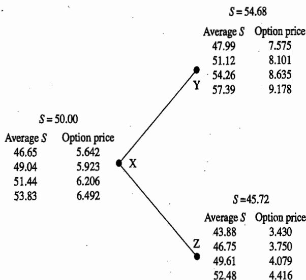
Figure 26.4 Part of tree for valuing option on the arithmetic average.
