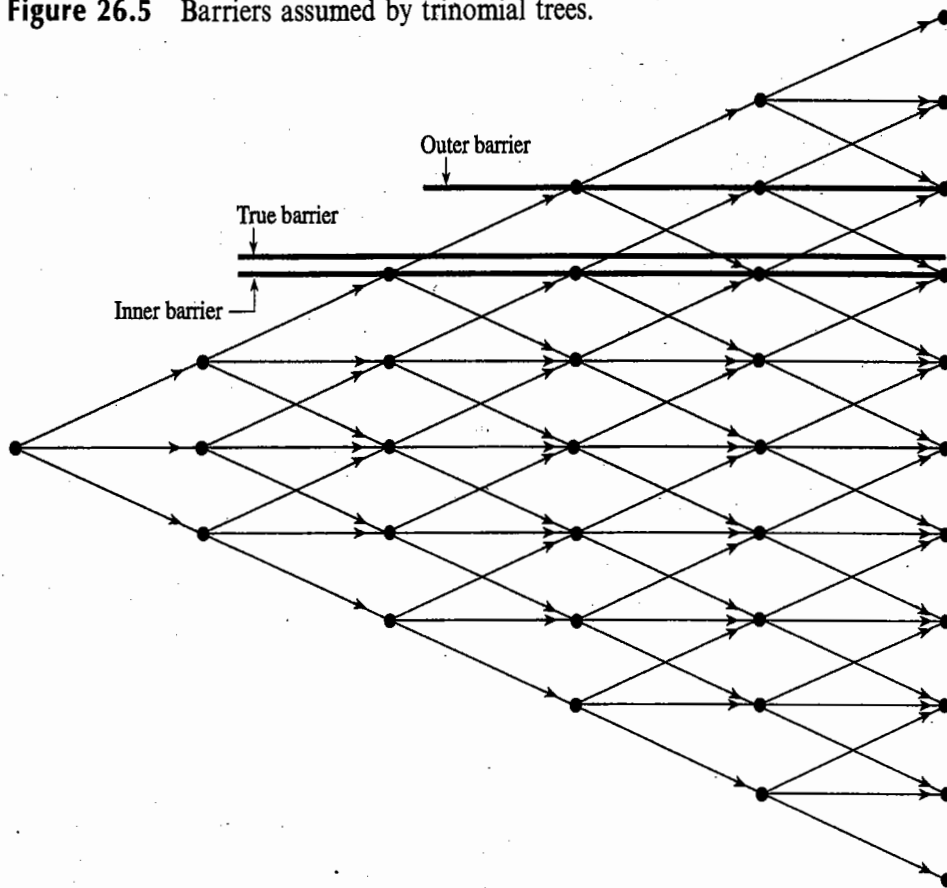
Figure 26.5 Barriers assumed by trinomial trees.
