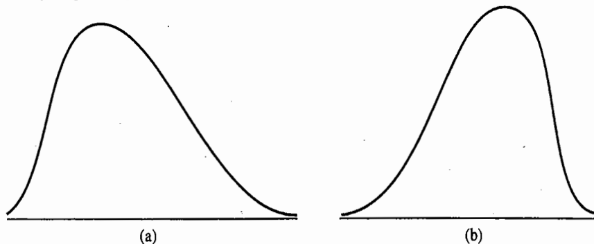
Figure 20.3 Probability distribution for value of portfolio: (a) positive gamma; (b) negative gamma.
