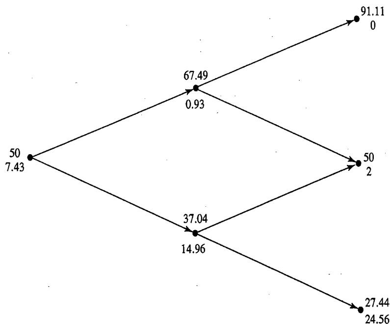
Figure 11.10 Two-step tree to value a 2-year American put option when the stock price is 50, strike price is 52, risk-free rate is 5%, and volatility is 30%.
