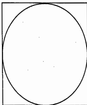
Figure 19.13 Calculation of \pi by throwing darts.
