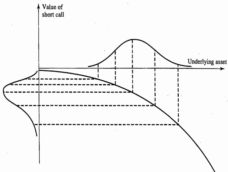
Figure 20.5 Translation of normal probability distribution for asset into probability distribution for value of a short call on asset.
