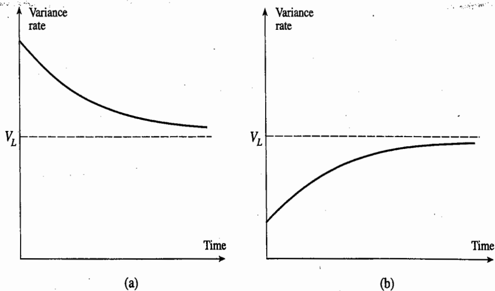
Figure 21.2 Expected path for the variance rate when (a) current variance rate is above long-term variance rate and (b) current variance rate is below long-term variance rate.
