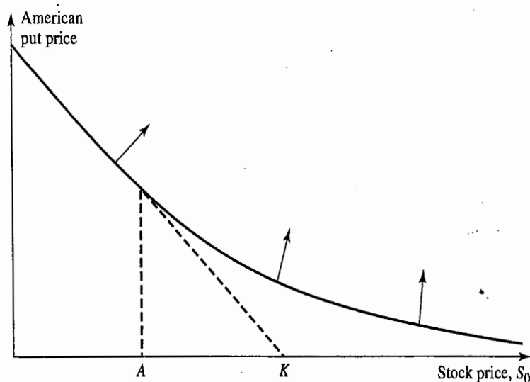
Figure 9.4 Variation of price of an American put option with stock price, S_0 .
