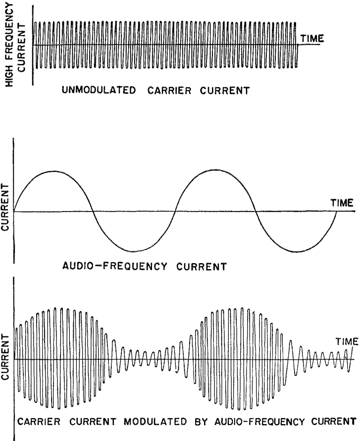
Figure 65. An amplitude-modulated carrier wave
