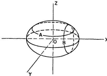
Figure 45. Two-dimensional sections of the ellipsoid
