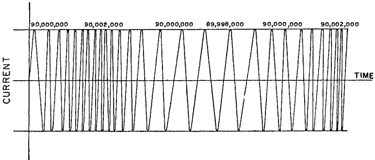
Figure 66. A frequency-modulated carrier wave
