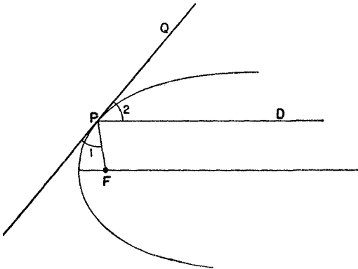
Figure 40. The focusing property of a parabola
