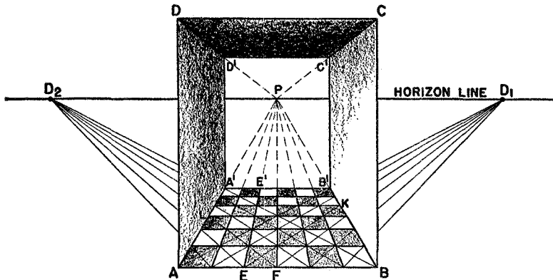
Figure 23. Sketch of a hallway according to the focused system of perspective
