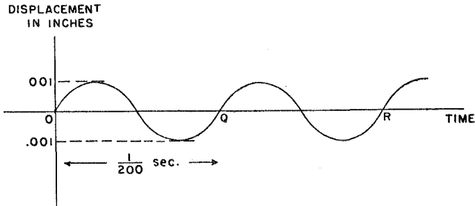
Figure 55. Graph of displacement versus time of a typical molecule of air
