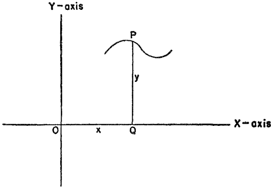
Figure 37. The rectangular co-ordinate system
