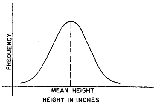
Figure 71. The normal frequency curve
