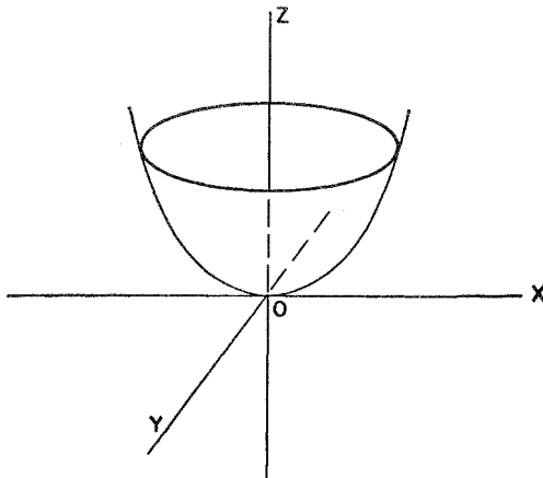
Figure 44. The paraboloidal surface corresponding to x^2 + y^2 = z
