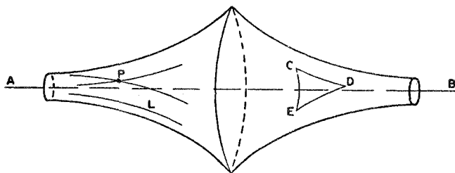
Figure 81. Pictorial interpretation of Lobatchevsky's and Bolyai's non-Euclidean geometry
