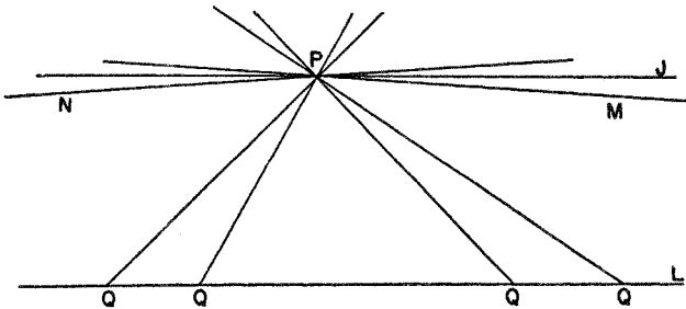
Figure 79. The parallel axiom of Lobatchevsky and Bolyai
