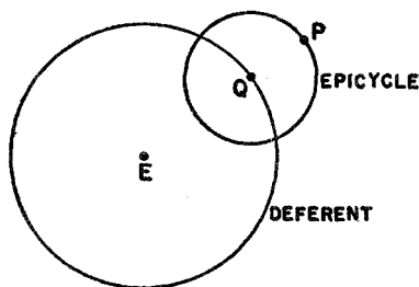
Figure 17. Sketch of Hipparchus' scheme
