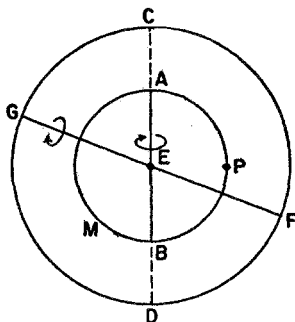
Figure 15. Sketch of the Eudoxian scheme
