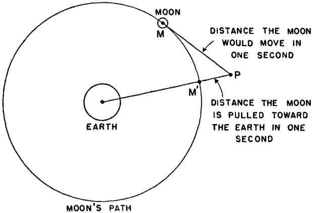
Figure 49. The gravitational effect of the Earth on the moon
