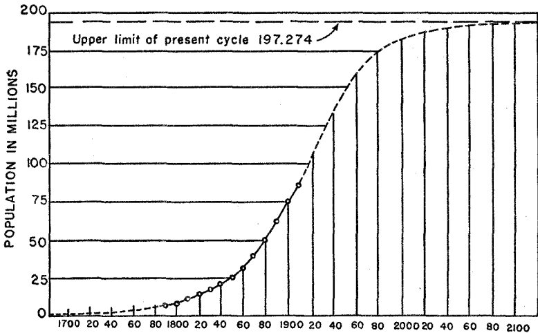
Figure 69. Growth of the population of the United States
