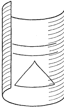
Figure 80. A new pictorial interpretation of Euclidean geometry
