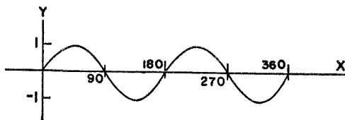
Figure 58. Graph of y = \text{sine } 2x
