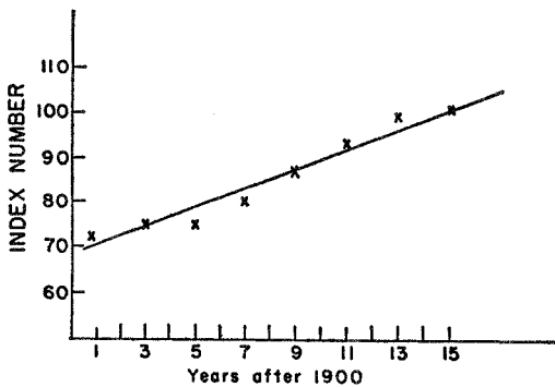
Figure 74. Graph of the data on food prices
