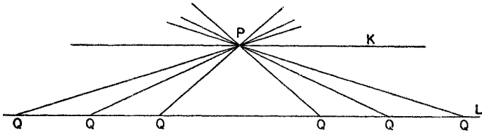
Figure 78. Euclid's parallel as a unique limiting line
