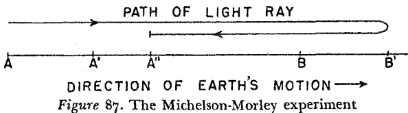
Figure 87. The Michelson-Morley experiment
