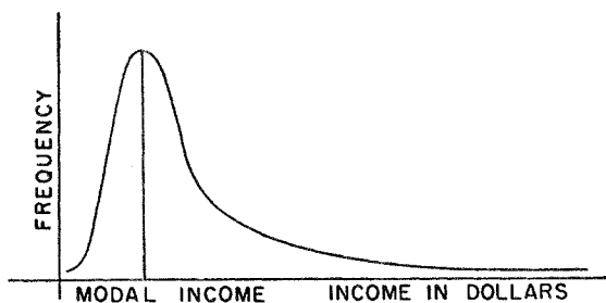
Figure 73. The frequency distribution of income
