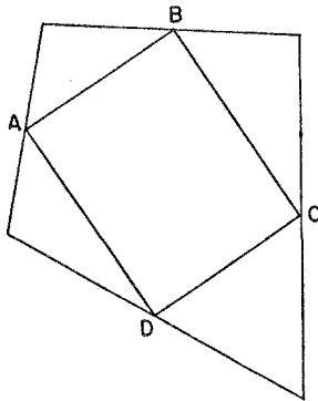
Figure 88. The lines joining the midpoints of the sides of any quadrilateral form a parallelogram
