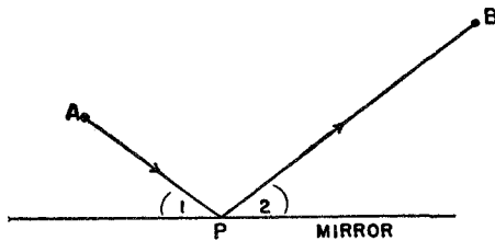
Figure 16. The angle of incidence equals the angle of reflection
