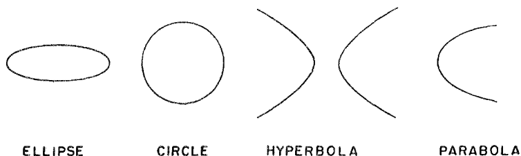
Figure 8. The conic sections
