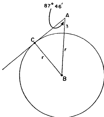
Figure 13. Calculation of the radius of the earth
