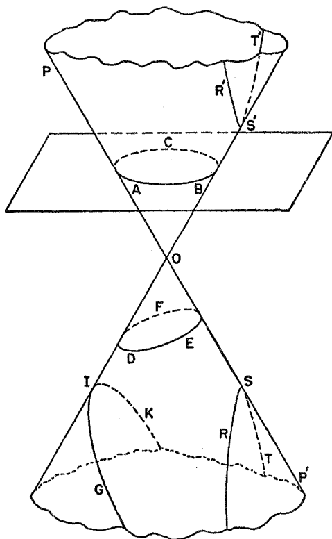
Figure 7. A conical surface and the sections made by intersecting planes
