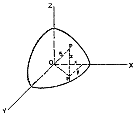
Figure 42. A sphere placed on a three-dimensional rectangular co-ordinate system
