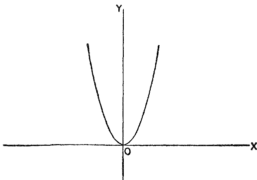
Figure 39. The curve of y = x^2
