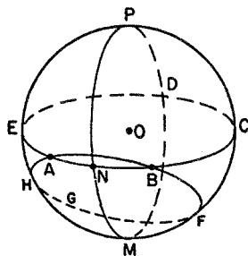
Figure 85. A pictorial interpretation of Riemann's geometry
