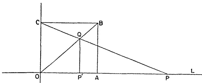
Figure 76. The one-to-one correspondence between the points of a unit segment and the points on a half-line
