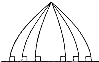
Figure 83. All the perpendiculars to a line meet in one point
