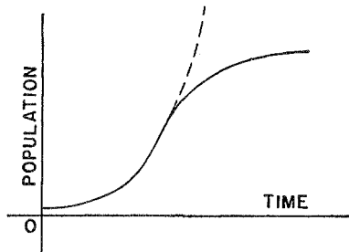
Figure 68. The curve of growth
