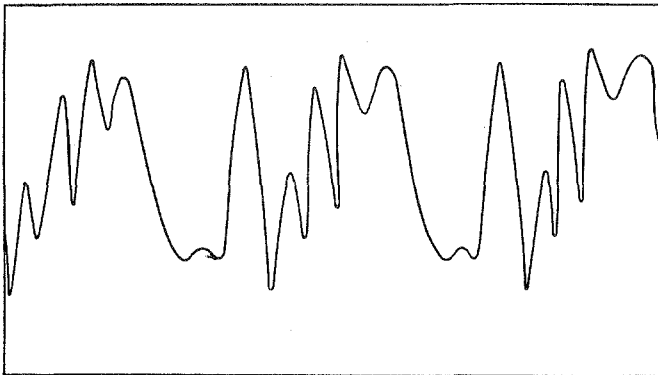
Figure 63. Tone of an oboe (Courtesy of Dayton C. Miller)
