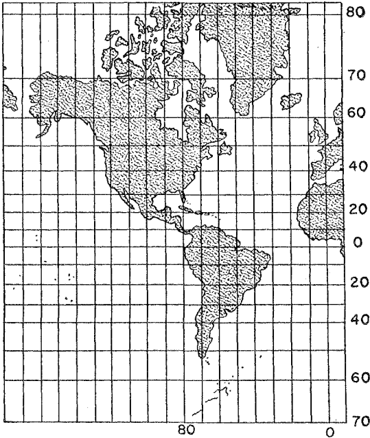
Figure 34. Mercator projection of the Western Hemisphere
