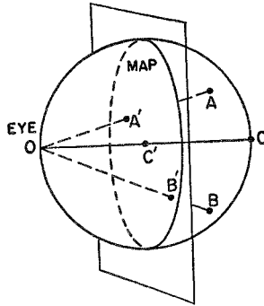
Figure 31. The principle of the stereographic projection
