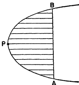
Figure 50. Area generated by a moving straight-line segment of variable length
