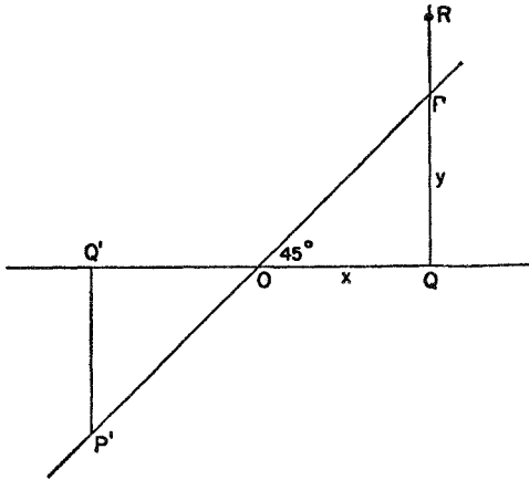
Figure 36. A straight line making a 45^\circ angle with the horizontal
