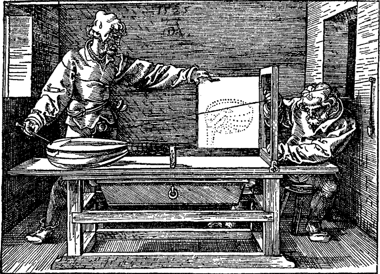
Figure 22. Dürer: The Designer of the Lute
