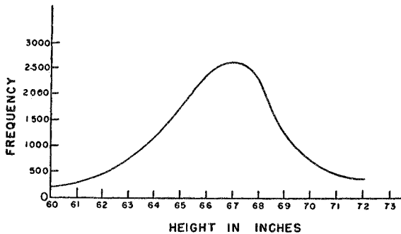
Figure 70. The heights of men in a certain community
