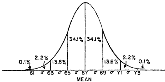
Figure 72. The percentages of cases falling in different regions of a normal frequency distribution
