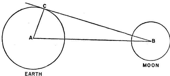
Figure 14. Calculation of the distance from the earth to the moon
