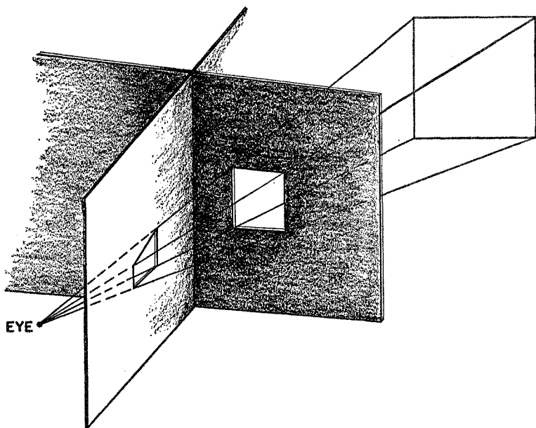
Figure 24. Two different sections of the same projection
