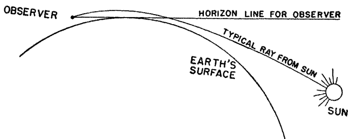
Figure 52. Light passing through a variable atmosphere takes the path requiring least time
