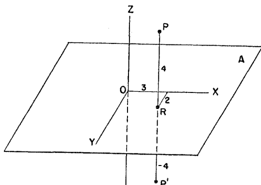
Figure 41. The three-dimensional rectangular co-ordinate system
