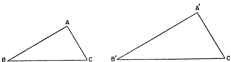
Figure 5. Two similar triangles
