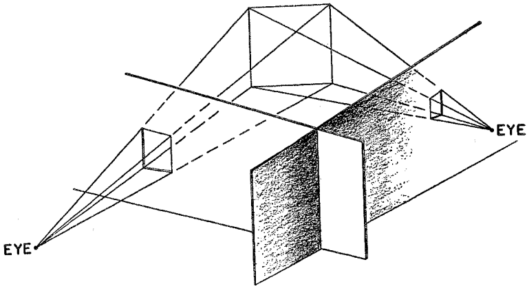
Figure 25. Sections of two different projections of the same scene
