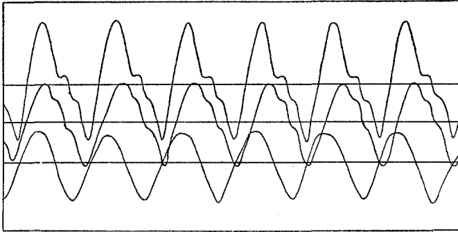
Figure 62. Different notes on the flute (Courtesy of Dayton C. Miller)
