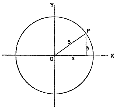
Figure 38. A circle placed on a rectangular co-ordinate system
