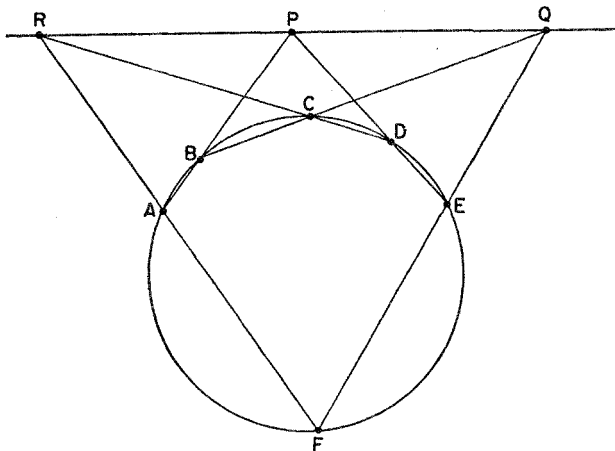
Figure 27. Pascal's theorem
