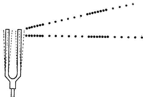
Figure 53. Motion of molecules of air due to a vibrating tuning fork
