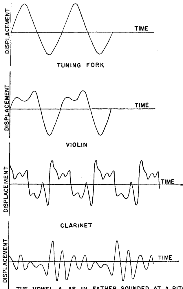
THE VOWEL A AS IN FATHER SOUNDED AT A PITCH OF 159 Figure 60. The periodicity of instrumental and vocal sounds (Courtesy of Dayton C. Miller)
