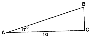
Figure 12. Calculation of the height of a mountain
