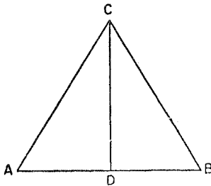
Figure 4. An isosceles triangle
