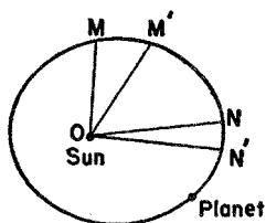
Figure 18. The elliptical and equal-area laws of planetary motion
