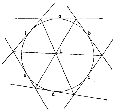
Figure 28. Brianchon's theorem
