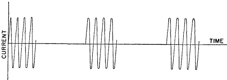
Figure 67. Radar pulses
