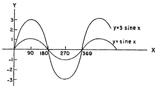
Figure 57. Graphs of y = \text{sine } x and y = 3 \text{ sine } x
