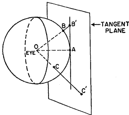
Figure 29. The principle of the gnomonic projection
