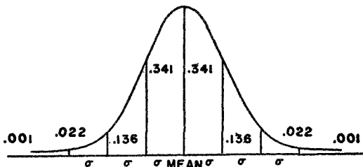
Figure 75. The normal probability curve
