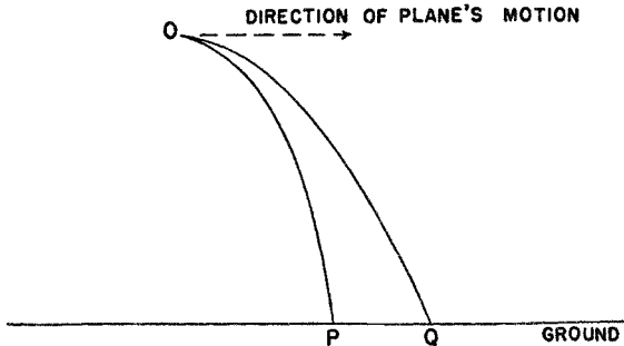
Figure 48. Two freely falling objects with different horizontal velocities reach the ground in the same time
