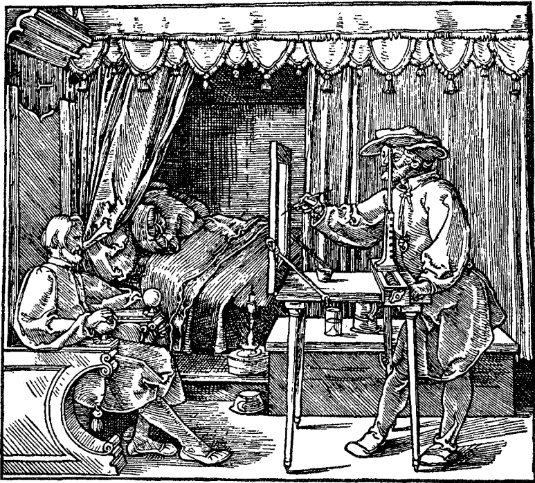
Figure 19. Dürer: The Designer of the Sitting Man
