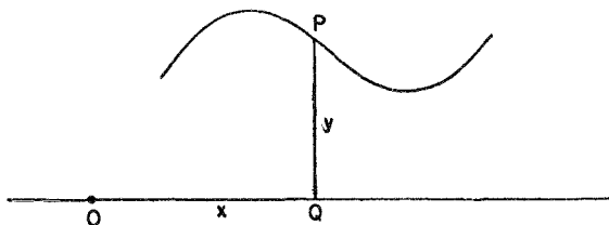
Figure 35. A curve generated by the motion of a straight-line segment of varying length
