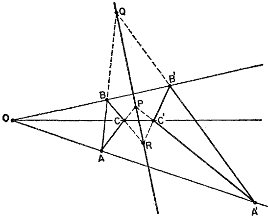
Figure 26. Desargues' theorem
