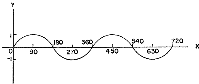
Figure 56. Graph of y = \text{sine } x
