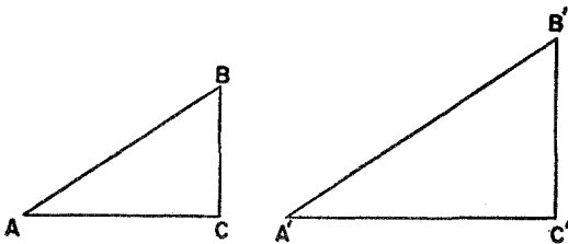
Figure 11. Two similar right triangles
