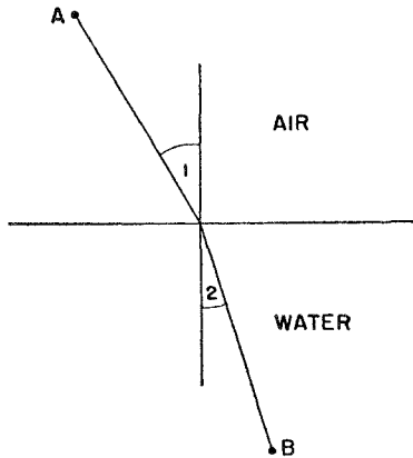
Figure 51. Refracted light takes the path requiring least time
