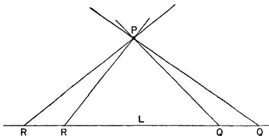
Figure 82. The geometrical basis for Riemann's parallel axiom
