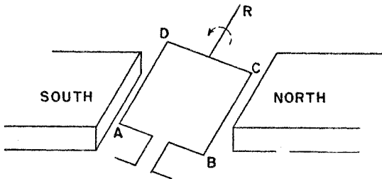
Figure 64. The principle of a generator of electricity
