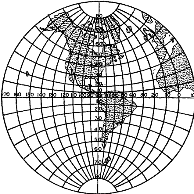
Figure 32. Stereographic map of the Western Hemisphere
