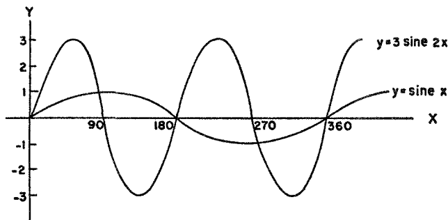
Figure 59. Graphs of y = \text{sine } x and y = 3 \text{ sine } 2x
