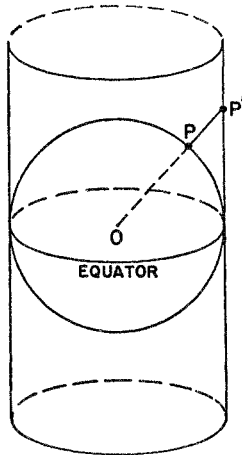
Figure 33. The principle of the perspective cylindrical projection
