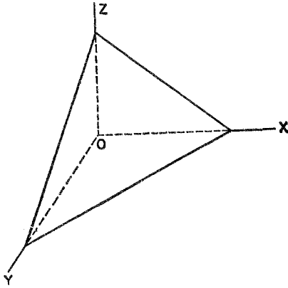
Figure 43. The plane corresponding to 3x + 4y + 5z = 6
