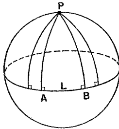
Figure 86. All the perpendiculars to a great circle on a sphere meet in one point
